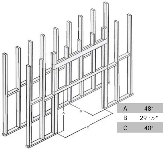
Framing Dimensions
