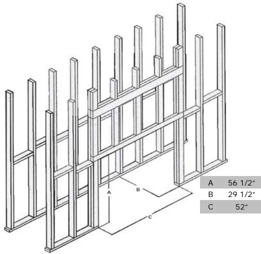
Framing Dimensions
