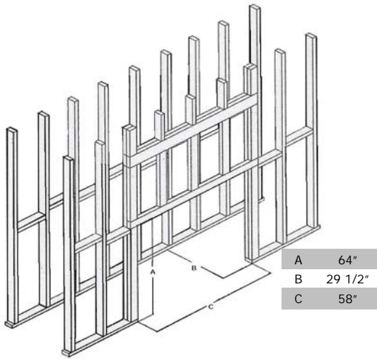
Framing Dimensions
