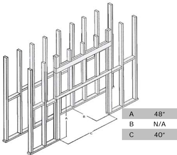
Framing Dimensions
