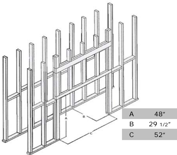
Framing Dimensions
